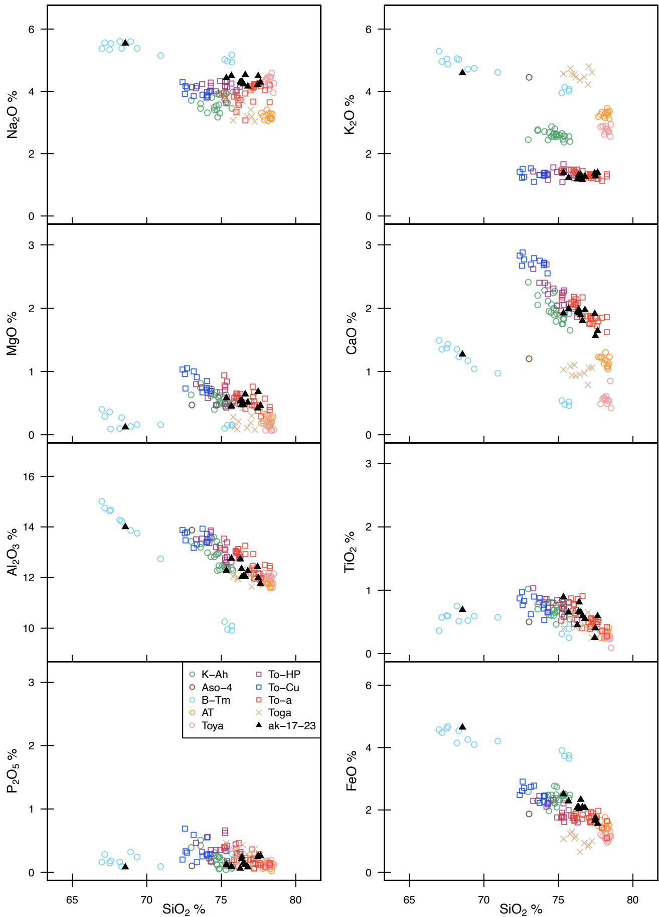
Bivariate plots for selected major elements of individual glass shards in ak-17-23
