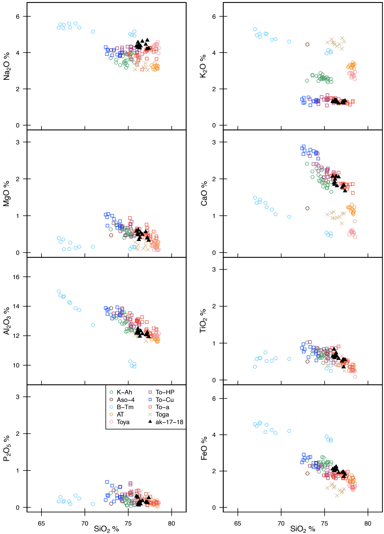
Bivariate plots for selected major elementss of individual glass shards in ak-17-18
