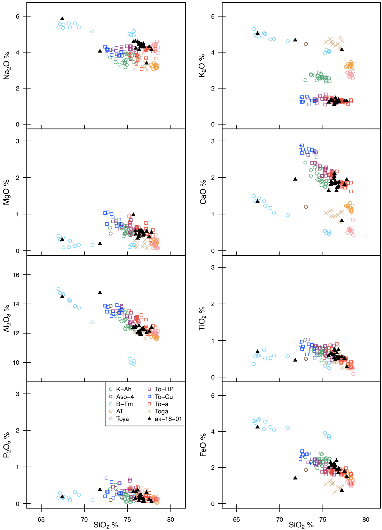
Bivariate plots for selected major elementss of individual glass shards in ak-18-01
