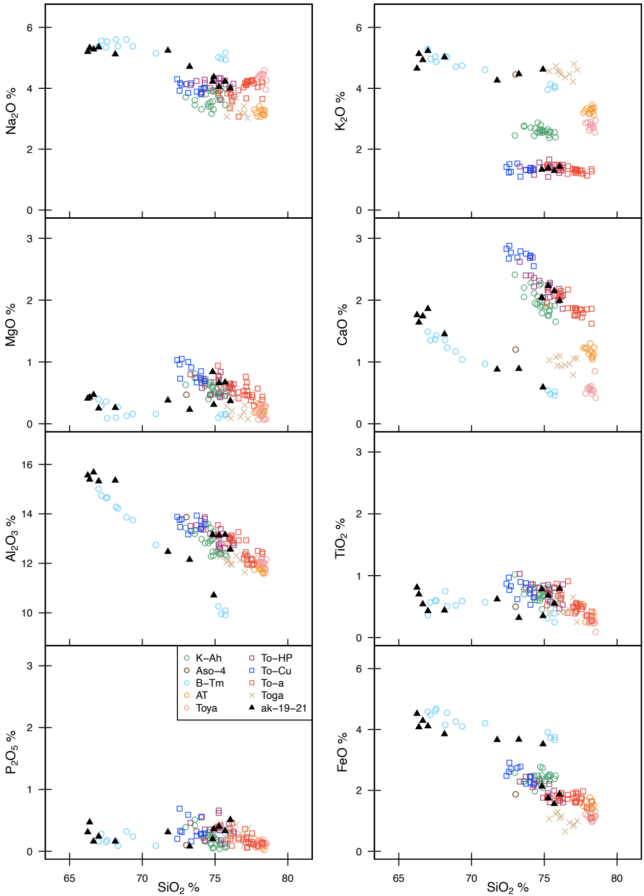
Bivariate plots for selected major elements of individual glass shards in ak-19-21
