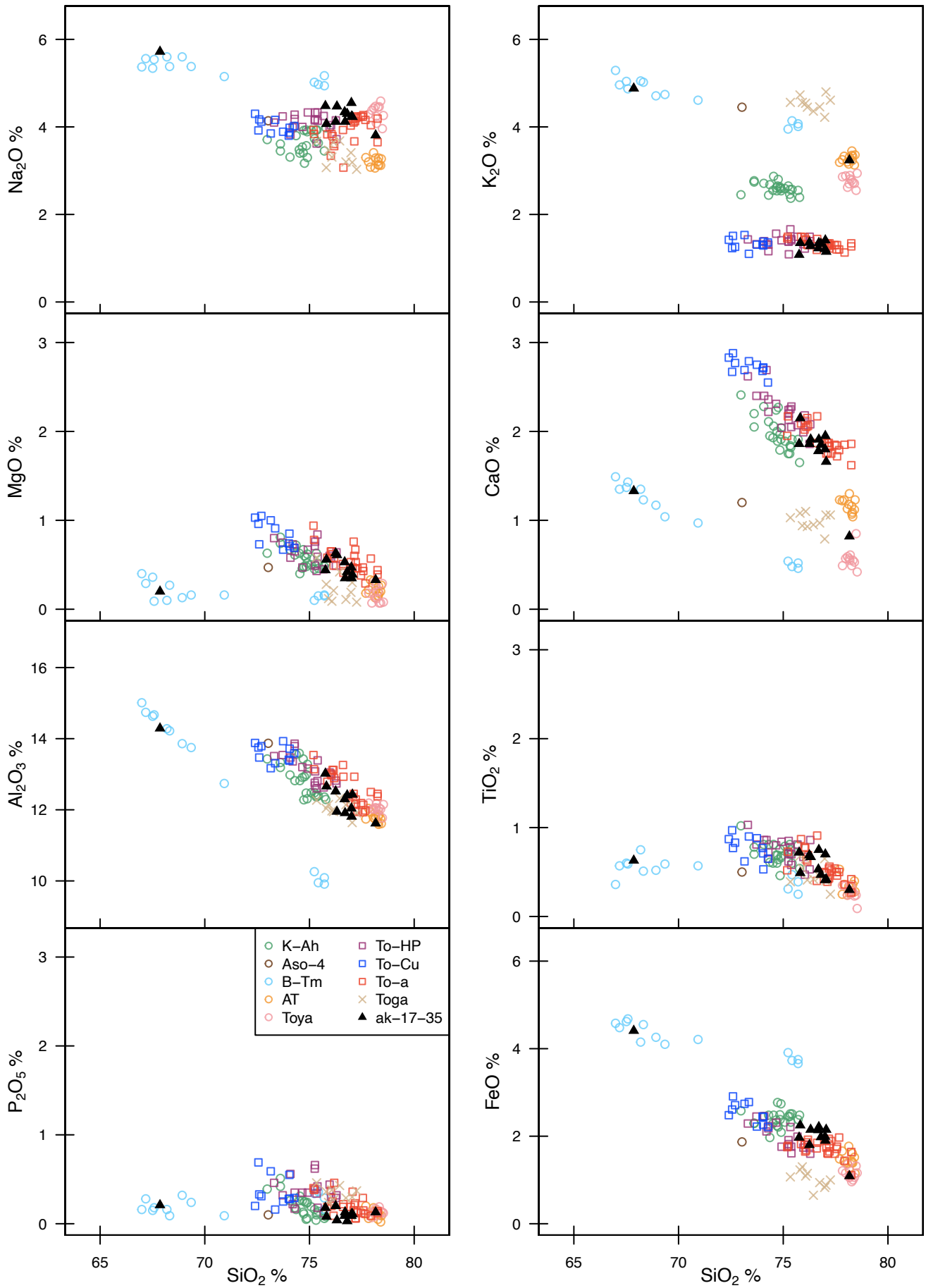
Bivariate plots for selected major elements of individual glass shards in ak-17-35
