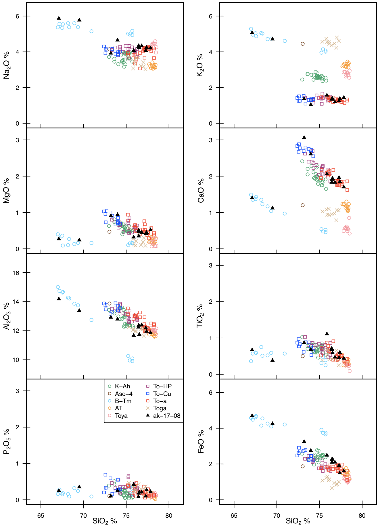
Bivariate plots for selected major elementss of individual glass shards in ak-17-08
