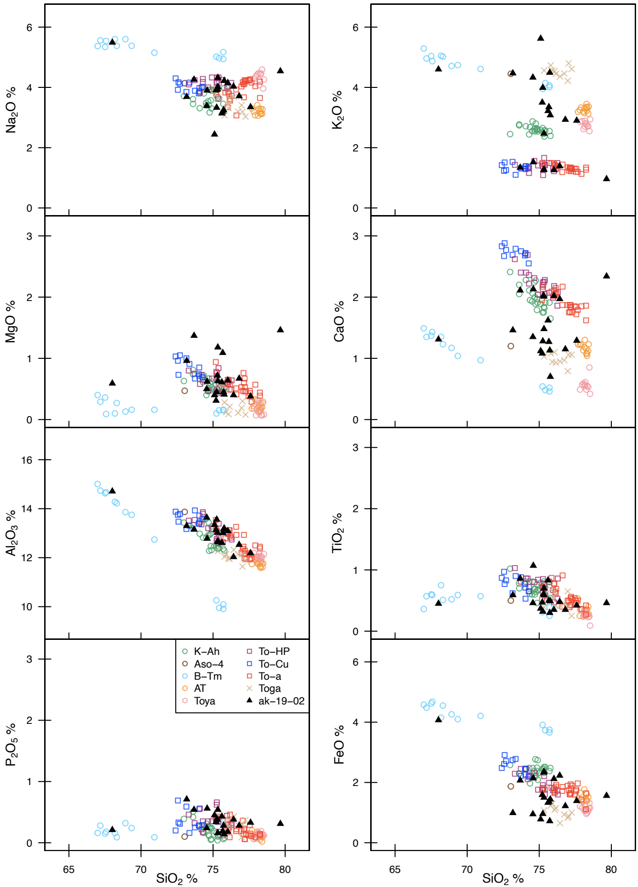
Bivariate plots for selected major elementss of individual glass shards in ak-19-02
