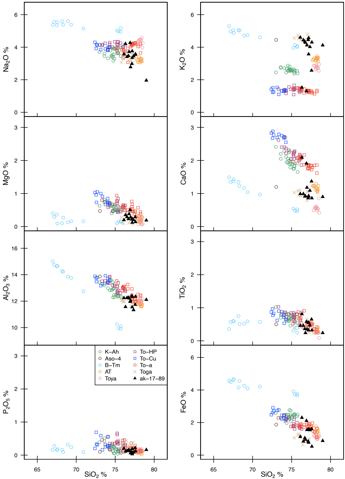
Bivariate plots for selected major elementss of individual glass shards in ak-17-89
