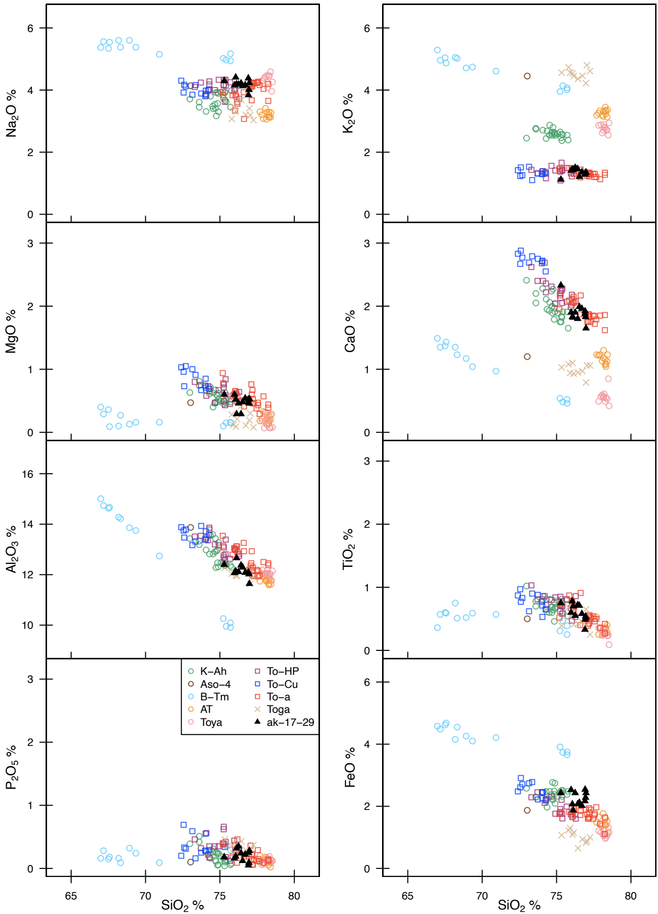
Bivariate plots for selected major elementss of individual glass shards in ak-17-29
